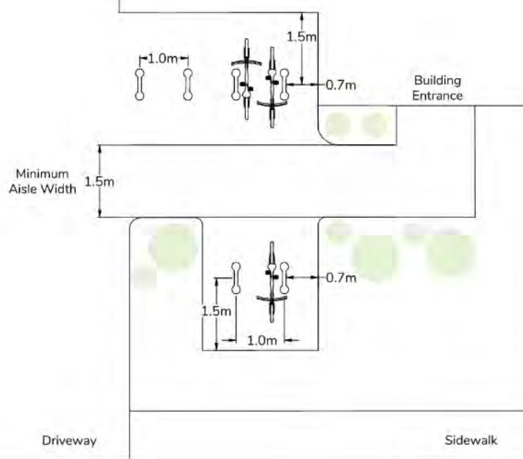
Figure 2: Short-Term Bicycle Parking Design
